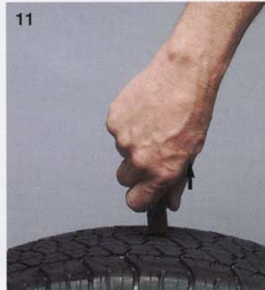
11 Pull Plugger and nozzle away from tire
