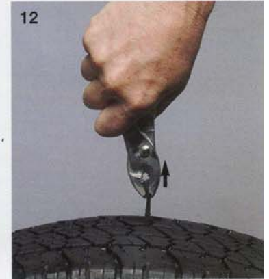
12 Use pliers to stretch the stem back toward you 2 inches
