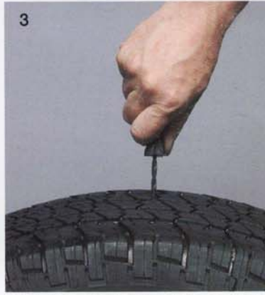
3 Thoroughly ream out hole with rasp tool
